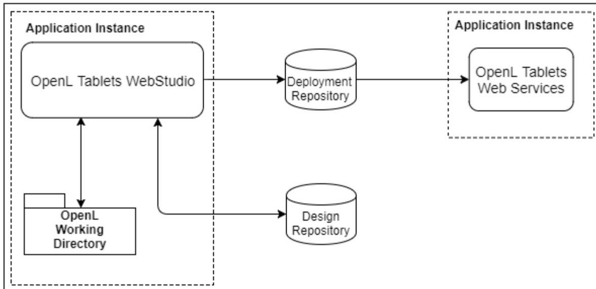
Figure 28: OpenL Tablets WebStudio and OpenL Tablets Rule Services deployment
