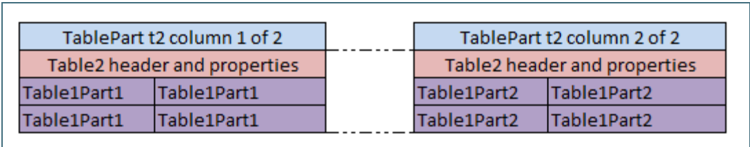
Figure 115: Horizontal merging of table parts
