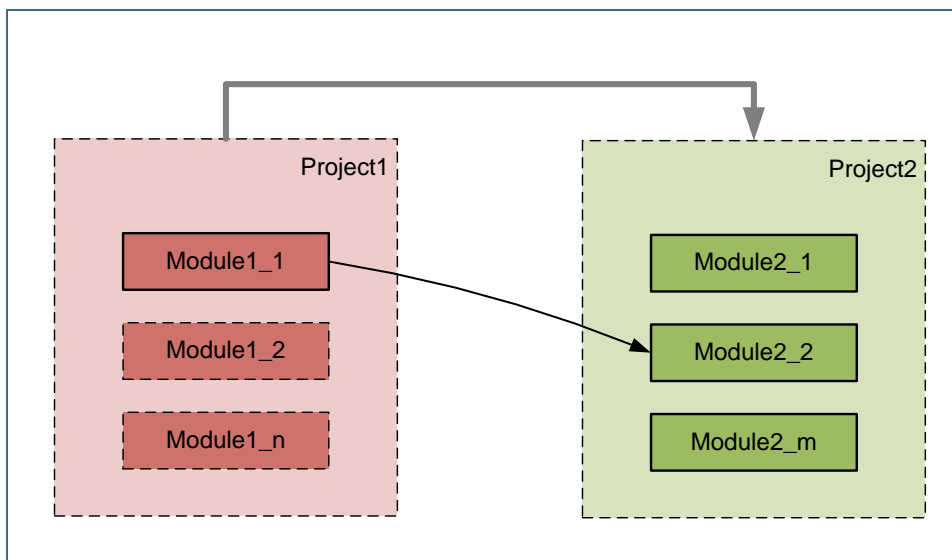
Figure 185: Example of a project and module dependencies combined
