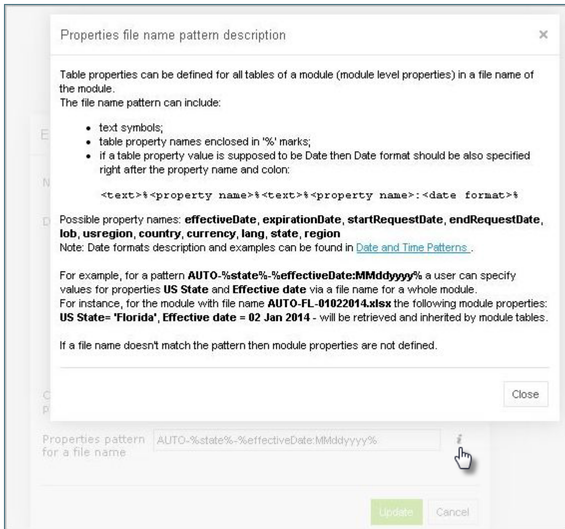
Figure 153: Properties file name pattern description
