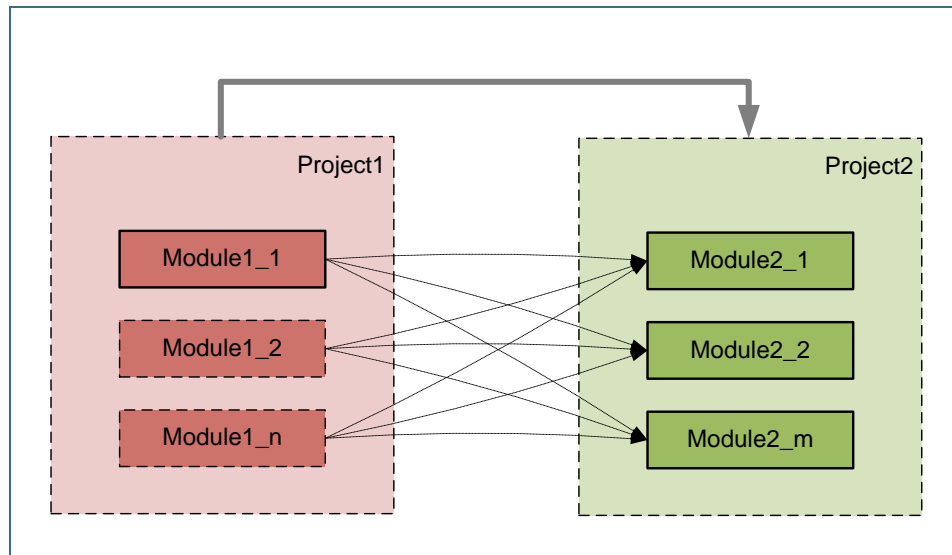
Figure 184: Interpretation of a project dependency (with all modules)
